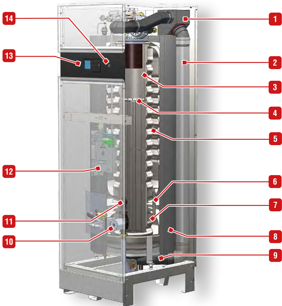
WaterMaster® 60 - 70 - 85 Evo 2
